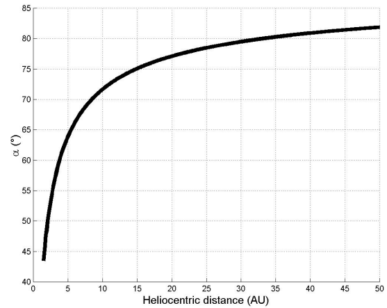
Figure 2: Stationary points vs. heliocentric distance.
