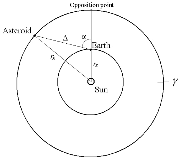
Figure1: Adopted geometry for the Sun-Earth-asteroid system.
